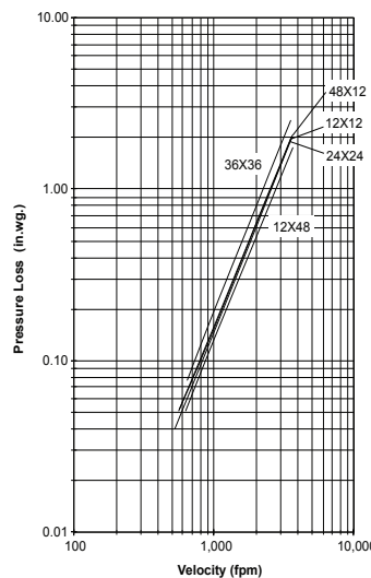
Figure 5.5 Plenum Mount
