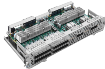
Multi-Port QSFP Line Card Board
