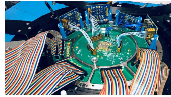
Chipset & Wafer Test Boards
