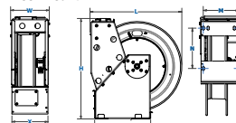
Floor Mount
