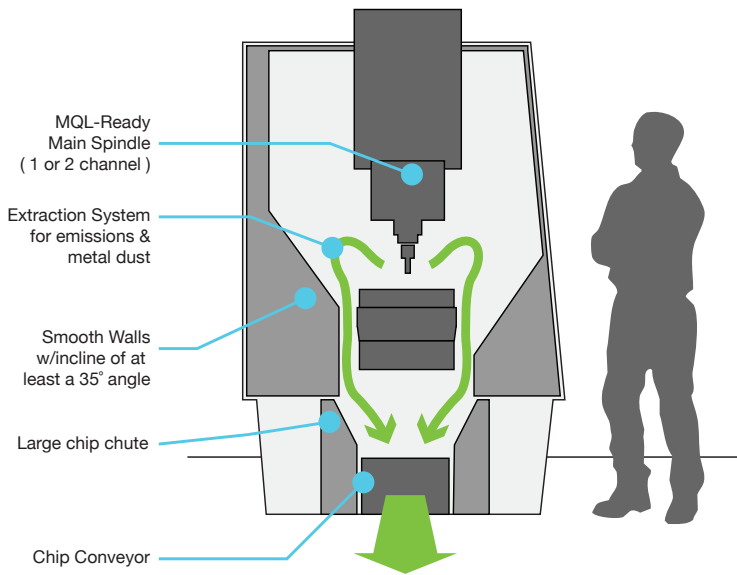
Figure 22: Elements of an MQL-specific machining center
