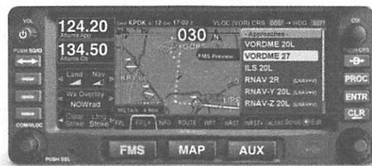
Figure 4: IFD4XX Unit
