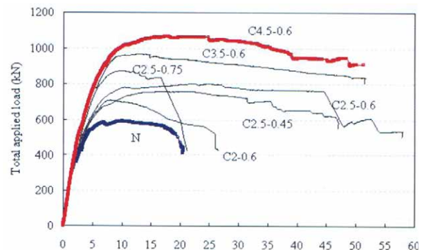
↑ The shear reinforcement effect of beam close-type-settlement (Closed type) T-shape beam (Ductile Failure)
