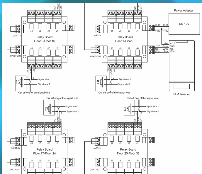
WIRING DIAGRAM
