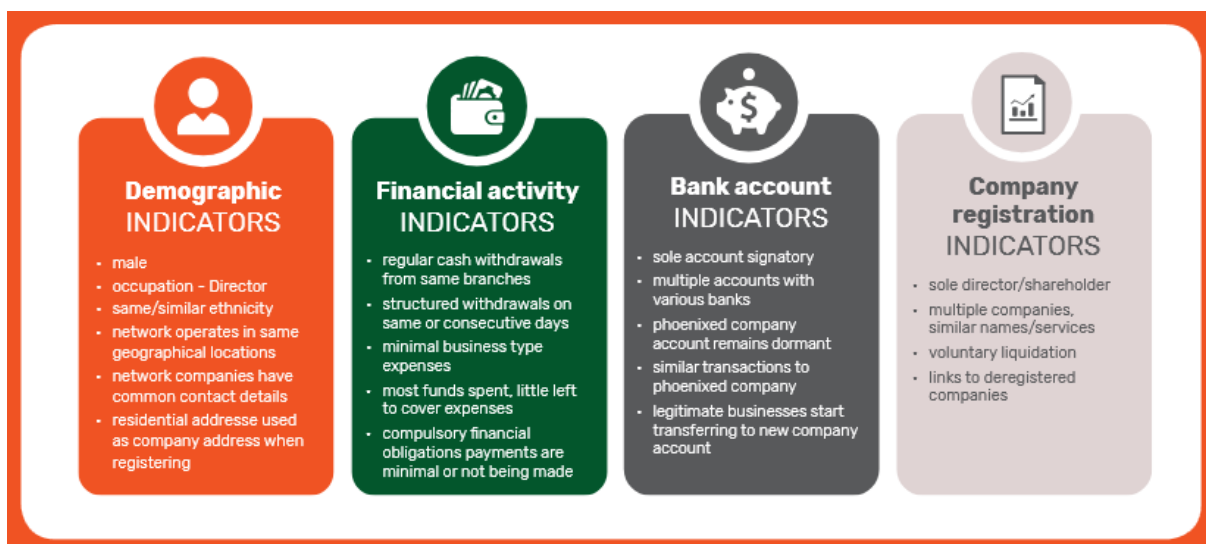
Figure 1: Phoenixing Indicators [9]
