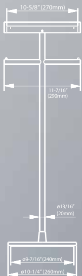
NEOREST REMOTE CONTROL STAND; YS990
