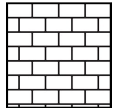
Runningbond Brick: 7.5" x 3.375" Grout: 1/2" 480 sqft per box
