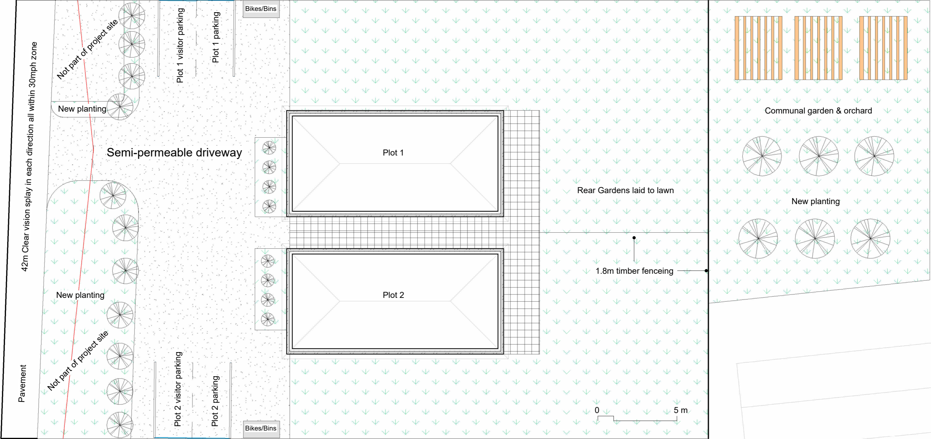
1 Site Plan Proposed - Detail 1 : 150
