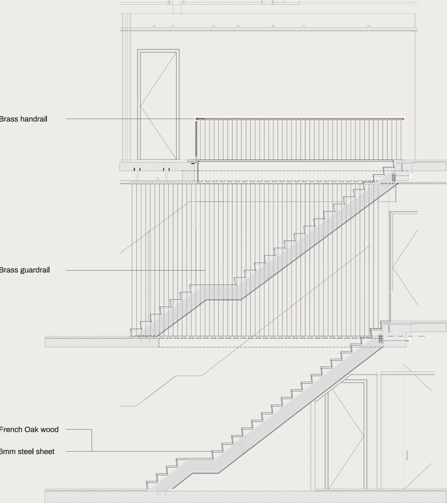
brass, steel and wood staircase section
