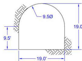
TAILRACE DISCHARGE TUNNEL
