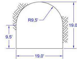
DISCHARGE WATER TUNNEL
