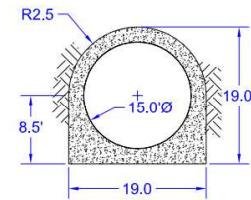
INTAKE TUNNEL DOUBLE BRANCH STEEL PIPE & (PC)
