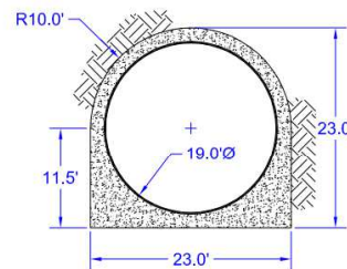
INTAKE TUNNEL SINGLE BRANCH STEEL PIPE & (PC)
