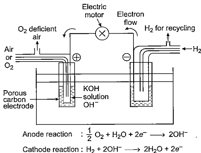
Fig. 5. Production of electricity from hydrogen.
