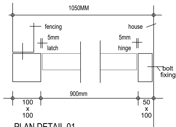
PLAN DETAIL 01
