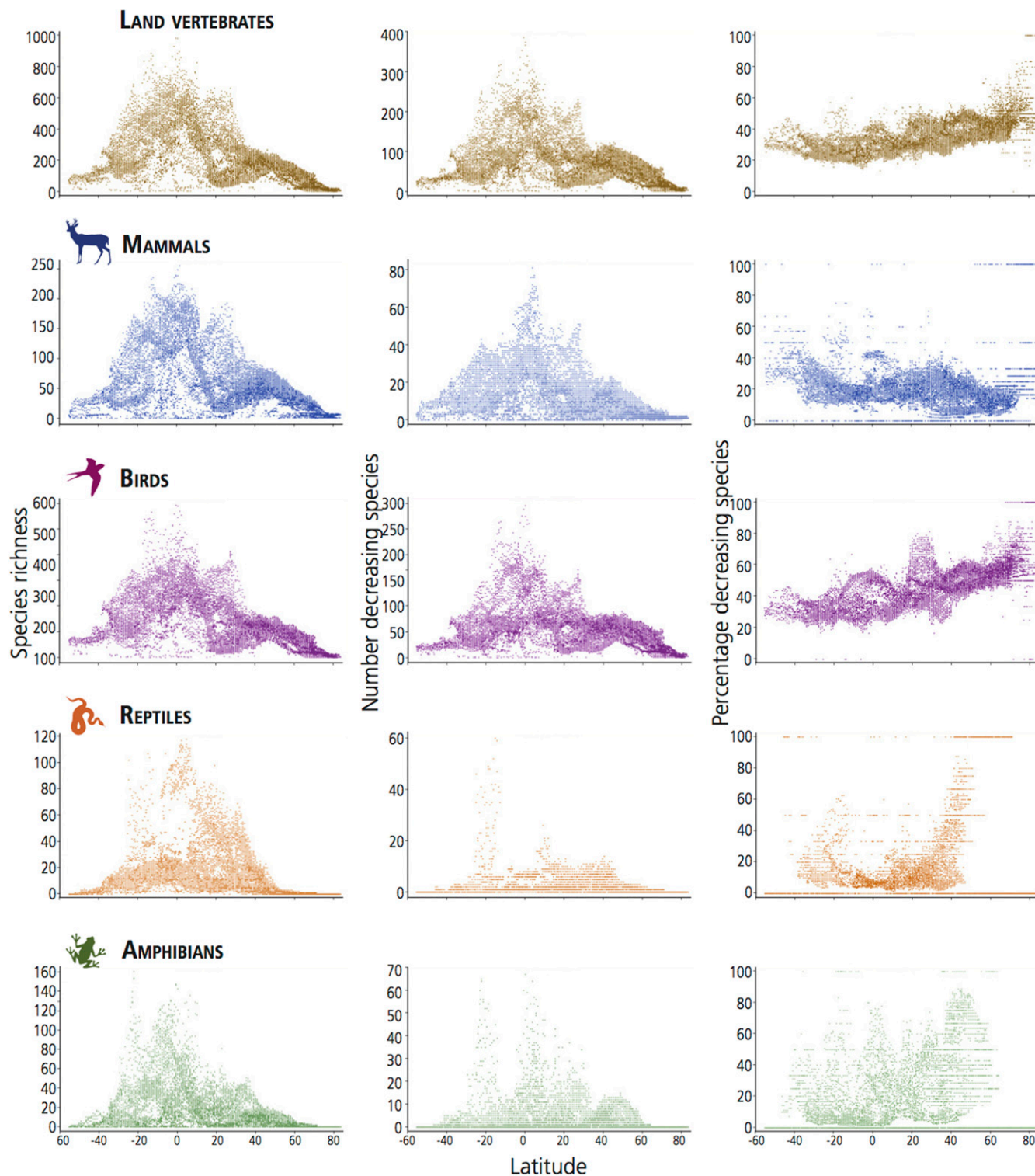
Fig. 3. Latitudinal distribution of species richness ( Left ), decreasing species ( Center ), and the percentage of species ( Right ) that are suffering population losses in relation to total species richness, in each 10,000-km 2 quadrat. Patterns of species richness in relation to latitude are similar in all vertebrates, although there are more species per quadrat in birds and mammals and, as expected, a scarcity of reptiles and amphibians at high latitudes. The patterns of number of species with decreasing populations indicate that regions with high species richness also have high numbers of decreasing species, but the percentage of decreasing species in relation to species richness shows contrasting patterns between mammals and birds compared with reptiles and amphibians. In mammals and birds, the percentage of decreasing species is relatively similar in regions with low and high species richness. In contrast, there are proportionally more decreasing species of reptiles and amphibians in regions with low species richness.
