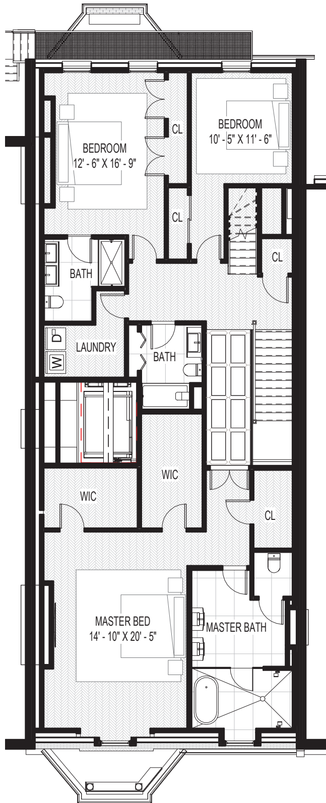
① UNIT 5 LEVEL 4 1" = 10'-0"
