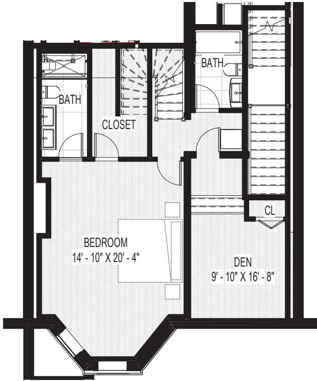
1 UNIT 1 GARDEN LEVEL 1" = 10'-0"
