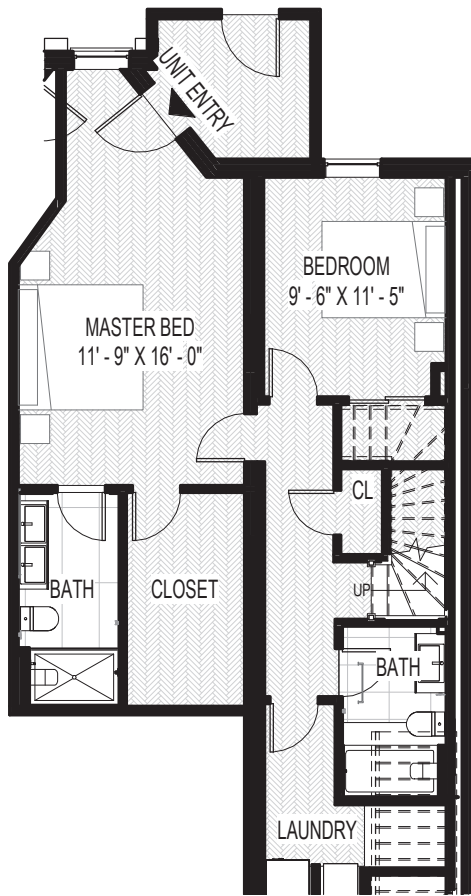
① UNIT 2 GARDEN LEVEL 1" = 10'-0"
