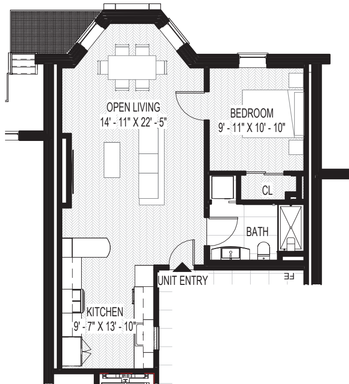
1 UNIT 4 LEVEL 2 1" = 10'-0"
