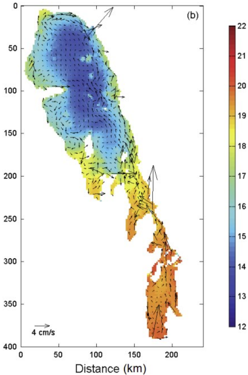
Simulated mean summer circulation & temperature average over depth
