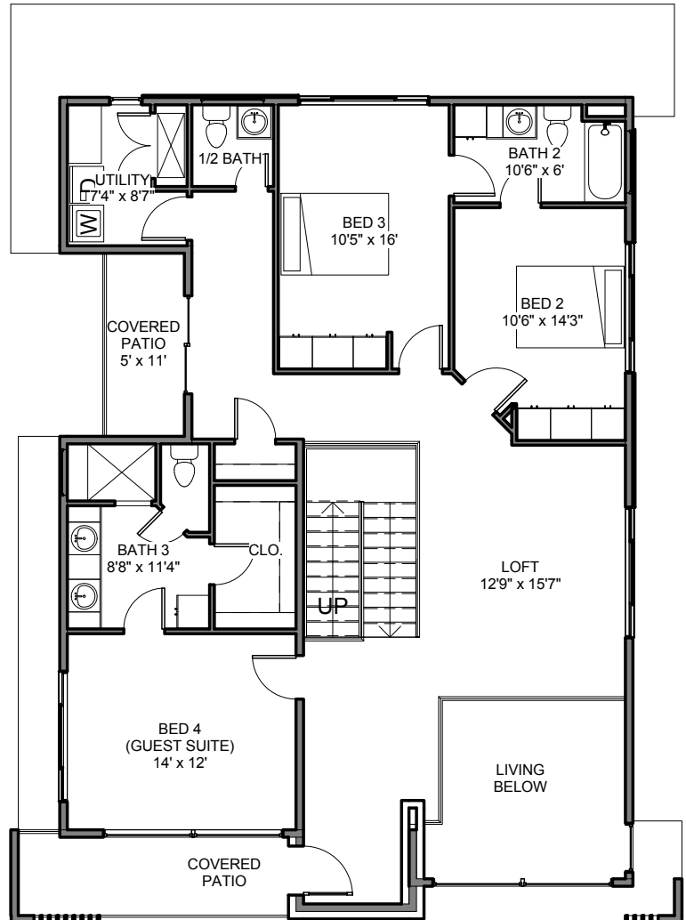
2nd FLOOR w. ADDITIONAL BED & LOFT
