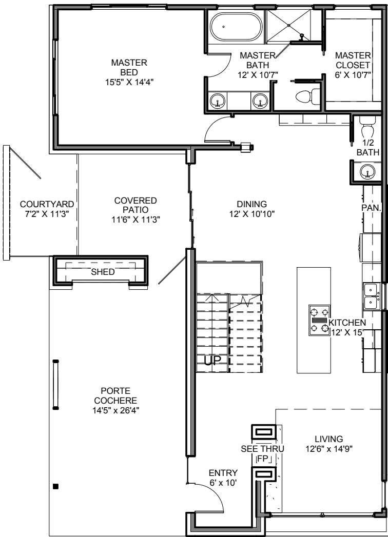
1st FLOOR PLAN w. SIDE ENTRY
