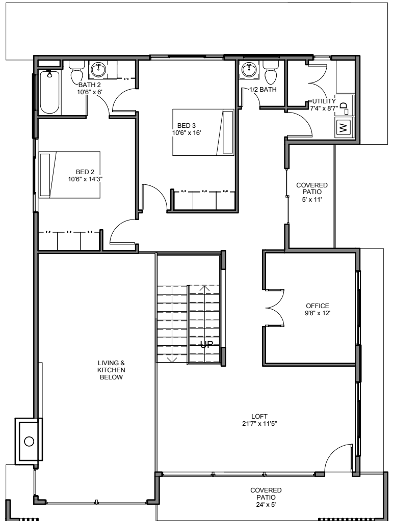
Second Floor
