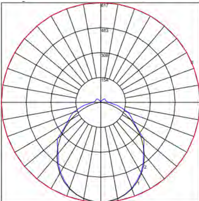
(Polar graph for 61LN40K48) Consult website of factory for files and photometrics
