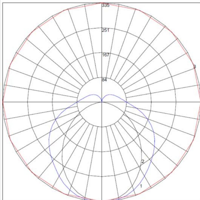
Maximum Candela = 334.88 Located At Horizontal Angle = 0, Vertical Angle = 0 # 1 - Vertical Plane Through Horizontal Angles (0 - 180) (Through Max. Cd.) # 2 - Vertical Plane Through Horizontal Angles (90 - 270) # 3 - Horizontal Cone Through Vertical Angle (0) (Through Max. Cd.)
