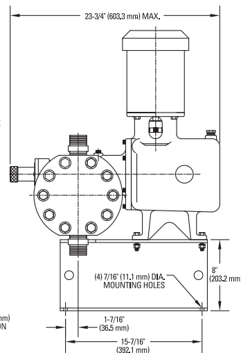
Models 635/637 (PVC & PVDF) Models 647 (All Materials)
