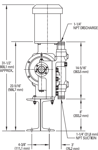
Model 647 (316SS & C-20 Heads)
