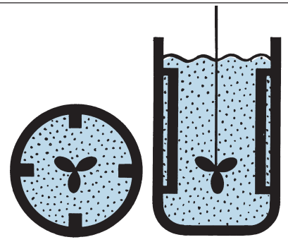
FIGURE 3 - For mixing in larger tanks, the mixer is often placed vertically on-center. In this configuration, baffles are recommended to prevent the contents of the tank from rotating, avoid vortexing and achieve good mixing and top-to-bottom turnover.
