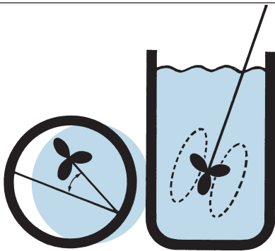
FIGURE 1 - Angling the portable mixer off-center is the position recommended by Neptune for rapid turnover of tank contents and good bottom washing.
