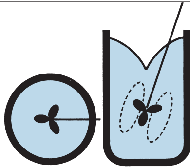
FIGURE 2 - On-center angling will produce good mixing with minimum vortexing. Tank contents turn over thoroughly but gently.
