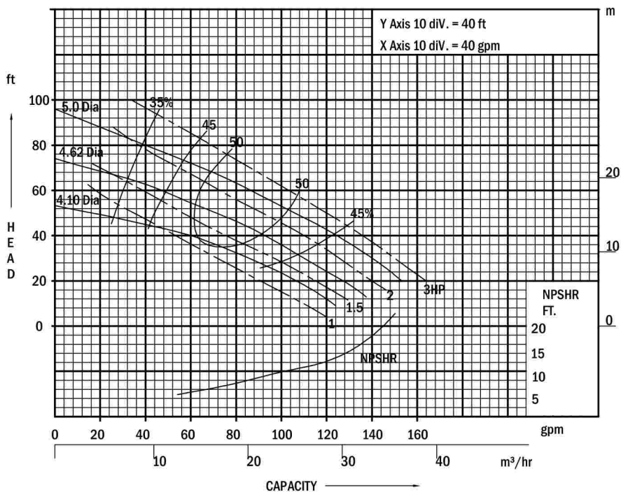
MODEL - SCP, Size - 2" x 2", RPM - 3450
