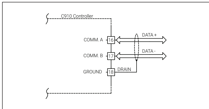
Fig. 2.10 – Communication Wiring (C910-485 only) RS-485 (2-Wire) Connections
