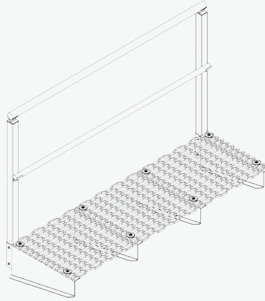
Levelled Walkway
