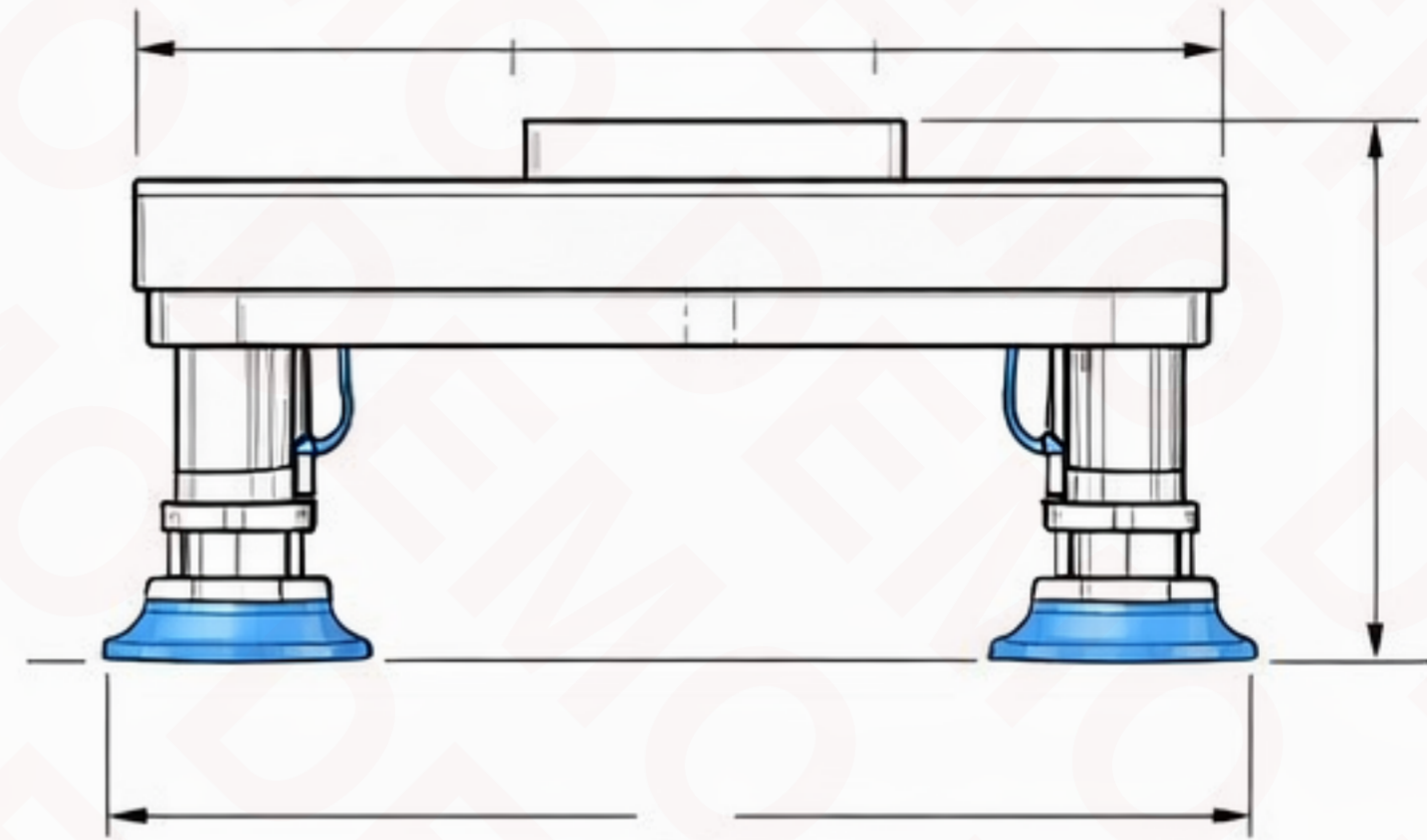
VISTA FRONTAL
