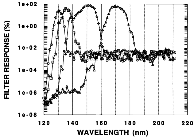
Fig. 4 Total response of the ultraviolet imager filters (log scale). Circles ( \circ ) represent response of O I line filter at 130.4 nm, squares ( \square ) response of O I line filter at 135.6 nm, diamonds ( \diamond ) response of LBH short-band filter, and triangles ( \triangle ) response of the filter for LBH long band.
