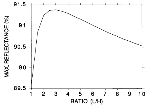
Fig. 1 Change in the calculated reflectance of a 35-layer \Pi multilayer as the optical thickness ratio ( L/H ) changes, where \text{MgF}_2 is used as the low ( L ) and \text{LaF}_3 as the high ( H ) refractive index material. The Koppelman limit for this case is 89.6%.
