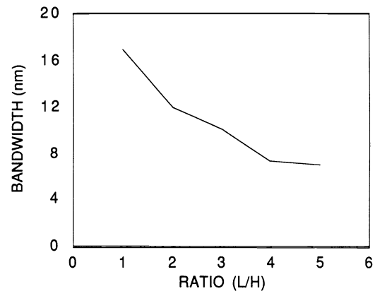
Fig. 2 Full width at half of the reflectance maximum of 35-layer \Pi stacks calculated for a 45-deg angle of incidence at 135.5 nm, where H represents optical thickness of a \text{LaF}_3 and L optical thickness of a \text{MgF}_2 film.
