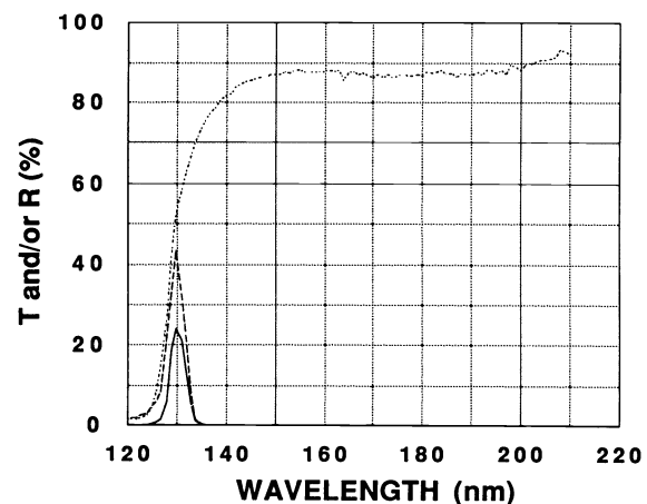
Fig. 3 Measured net transmittance (solid line) through three narrowband reflection filters (dashed line) centered at 130.4 nm and combined with the transmission filter (dotted line). The reflection filters operate at 45-deg angle of incidence. \text{MgF}_2 and \text{LaF}_3 are used as the low and high refractive index materials, respectively. The peak transmittance is greater than 22%, with 5-nm bandwidth. The average blocking for out-of-band wavelengths up to 2500 nm is better than 3 \times 10^{-3}\% with transmittance less than 10^{-6}\% at 121.6 nm (see Fig. 4).
