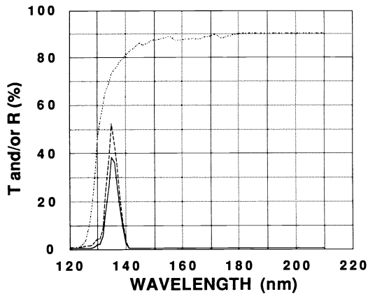
Fig. 5 Measured net transmittance (solid line) through three narrow-band reflection filters (dashed line) centered at 135 nm and combined with the transmission filter (dotted line). The reflection filters, which are designed using \text{MgF}_2 as the low and \text{LaF}_3 as the high refractive index materials, operate at 45-deg angle of incidence. The peak transmittance is greater than 38%, with 4.5-nm bandwidth. The average blocking for out-of-band wavelengths up to 2500 nm is better than 3 \times 10^{-3}\% with transmittance less than 10^{-6}\% at 121.6 nm (see Fig. 4).
