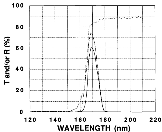
Fig. 7 Measured net transmittance (solid line) through three broad-band reflection filters (dashed line) centered at 170 nm and combined with the transmission filter (dotted line). The reflection filters operate at 45-deg angle of incidence. They are designed using \text{MgF}_2 as the low and \text{LaF}_3 as the high refractive index material. The peak transmittance is close to 60%, with 11-nm bandwidth. The average blocking for out-of-band wavelengths up to 2500 nm is better than 3 \times 10^{-3}\% with less than 5 \times 10^{-6}\% transmittance for wavelengths below 130 nm (see Fig. 4).
