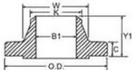
Weld Neck
