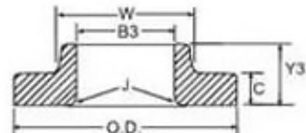
Lapped
