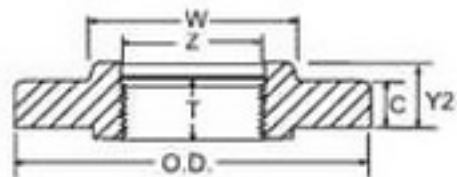
Threaded
