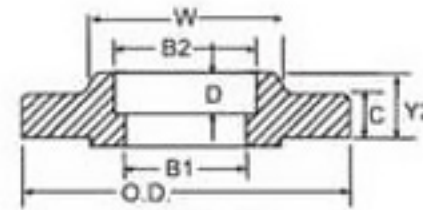
Socket Weld
