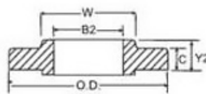
Slip-on
