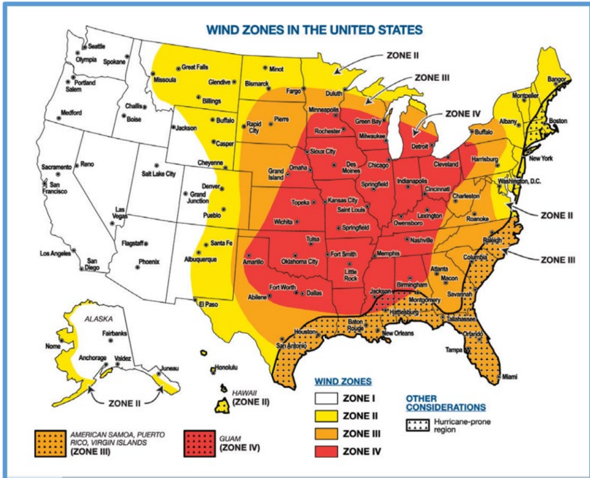
Figure 4.3.6-1: Wind Zones of the United States (IBEC, 2019)
