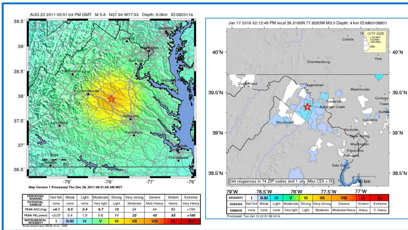
Figure 4.3.2-4: USGS ShakeMaps for August 2011 and January 2016 Earthquakes (USGS, 2016)
