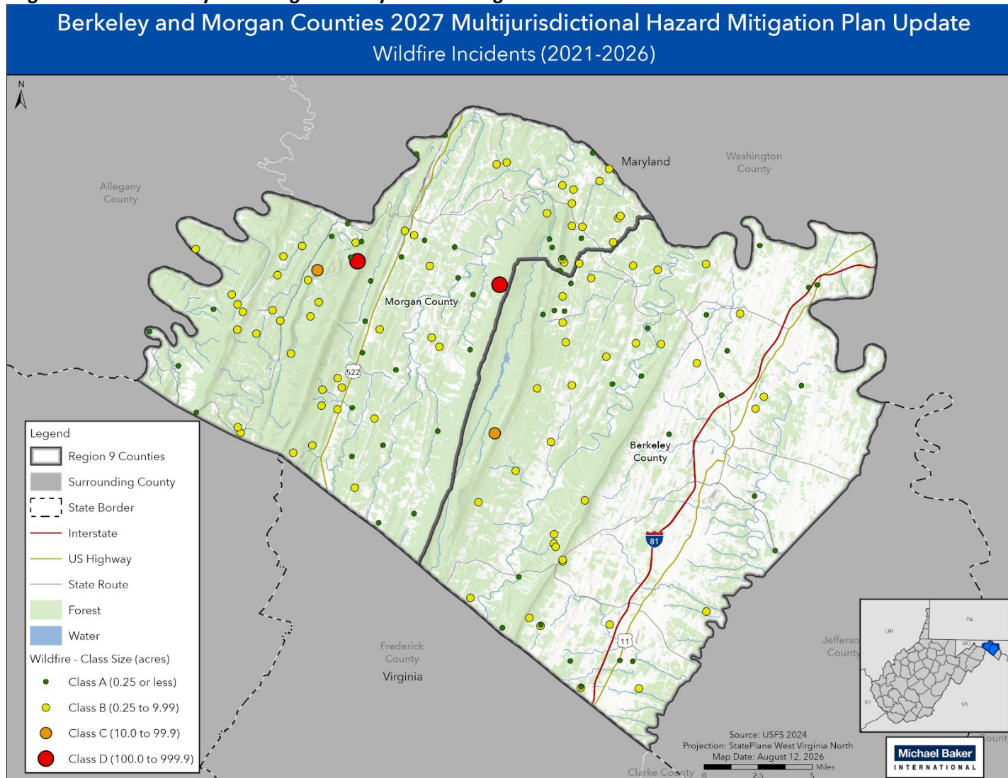
Figure 4.3.12-3 Berkeley and Morgan County Wildfire Origins
