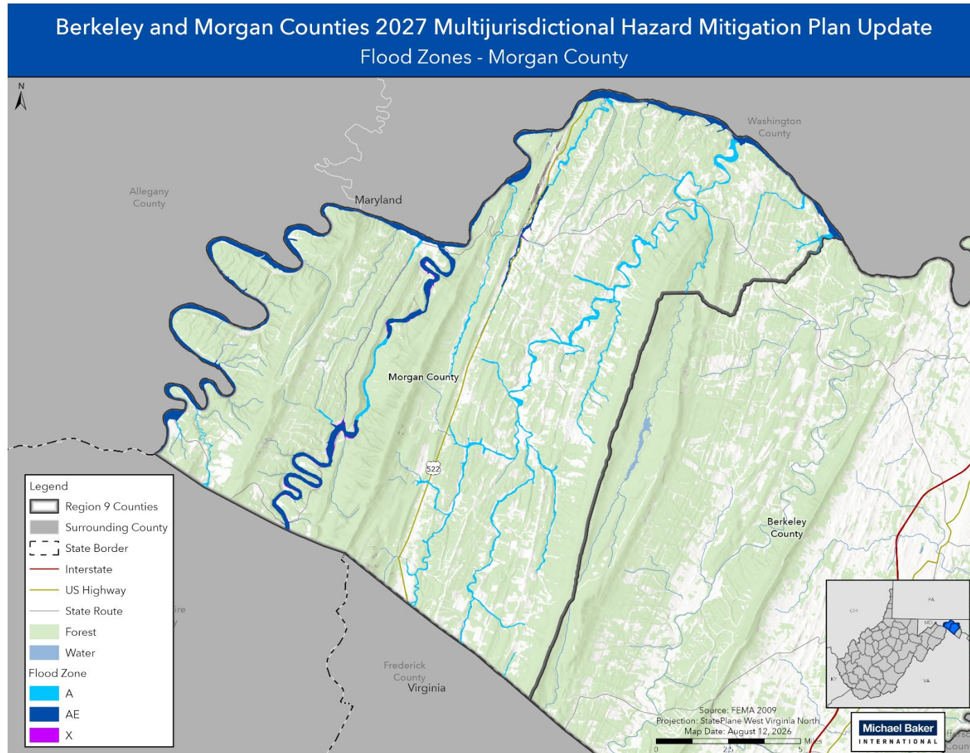
Figure 4.3.4-4: Flood Zones in Morgan County.
