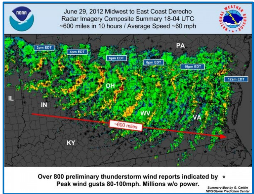
Figure 4.3.13-3: 6/29/12 Derecho Wind Storm
