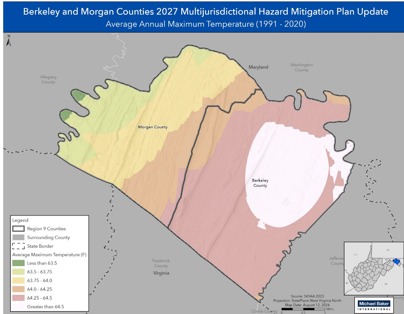
Figure 4.3.3-4: The Average Annual Maximum Temperature in Berkeley and Morgan Counties from 1991-2020.
