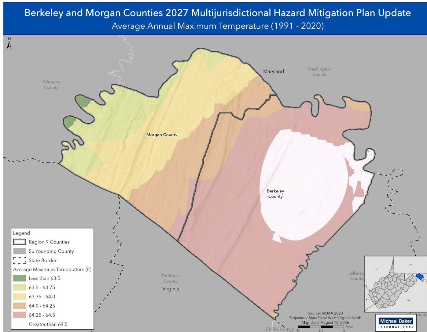
Figure 4.3.1-3 The Average Annual Maximum Temperature in Berkeley and Morgan Counties from 1991-2020.
