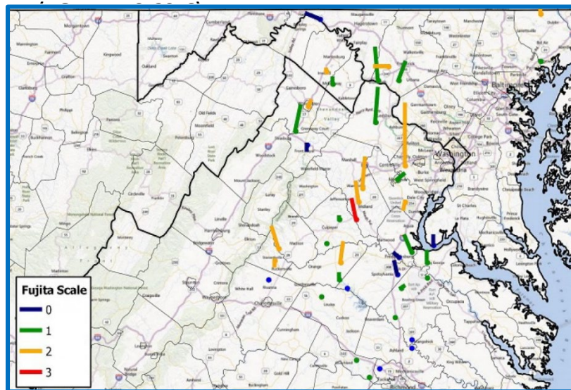
Figure 4.3.13-2 Tornado Tracks of Hurricane Ivan (Prociv, 2004)
