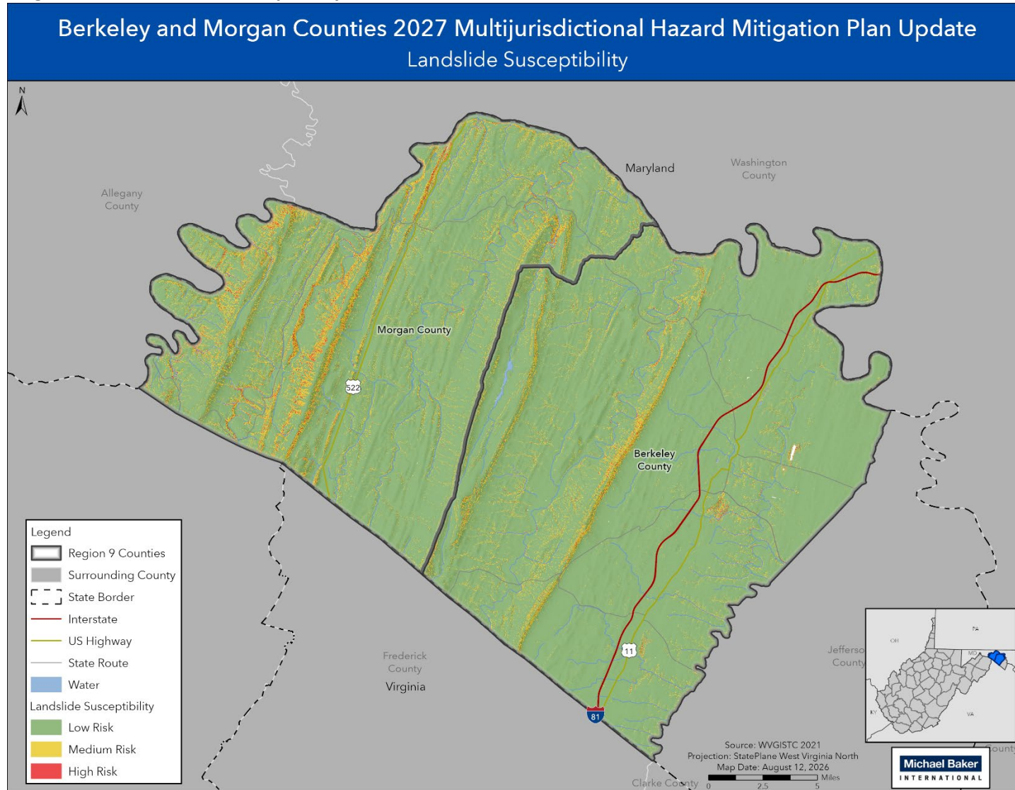
Figure 4.3.8-1 Landslide Susceptibility
