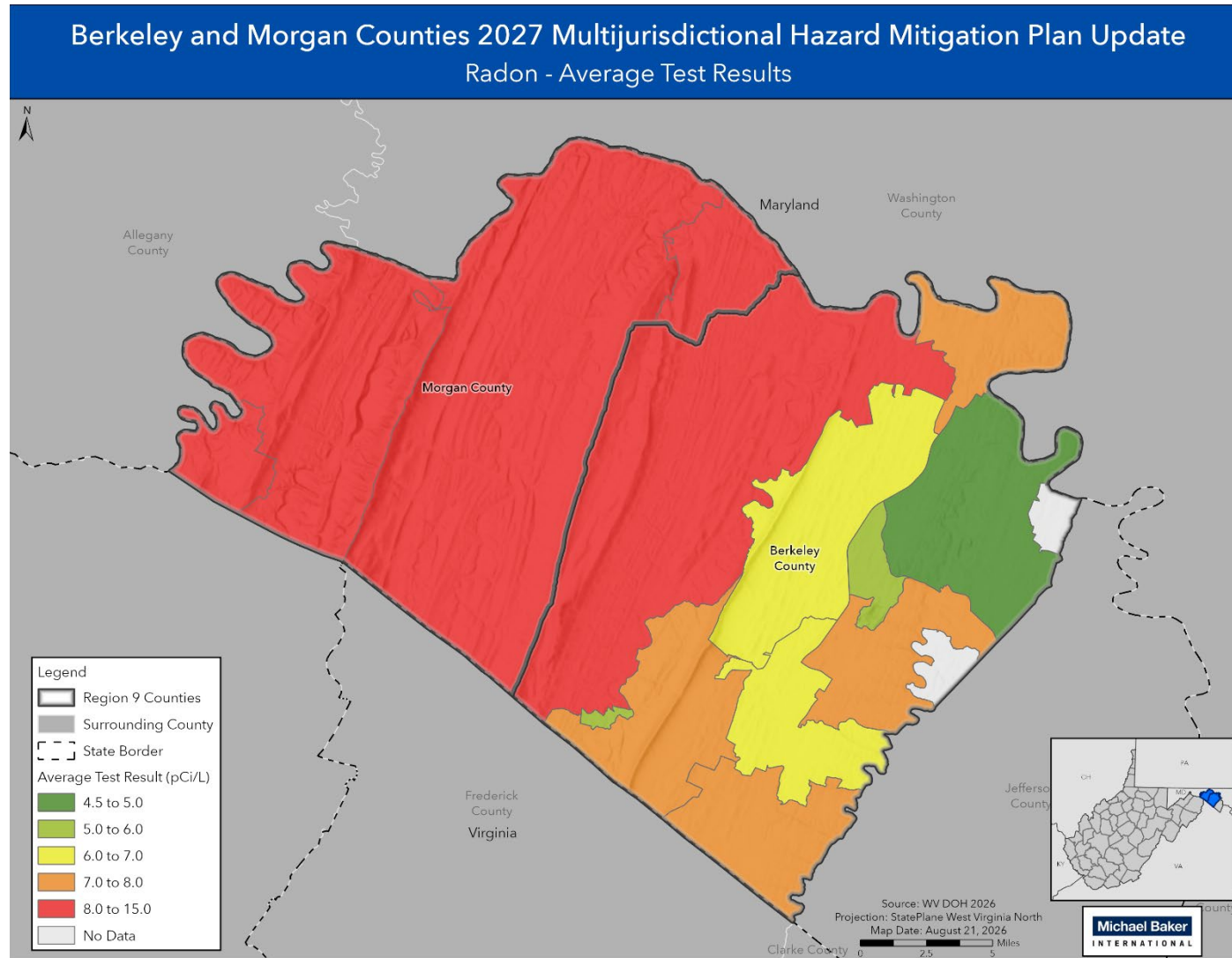
Figure 4.3.10-3 Average Radon Test Results for Berkeley and Morgan Counties
