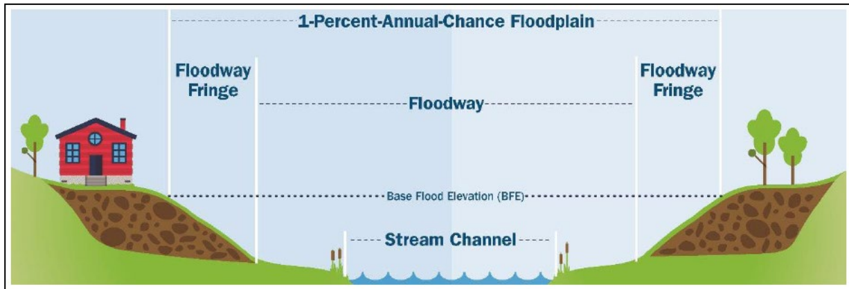
Figure 4.3.4-1: Diagram Identifying Special Flood Hazard Area and 100-Year Floodplain
