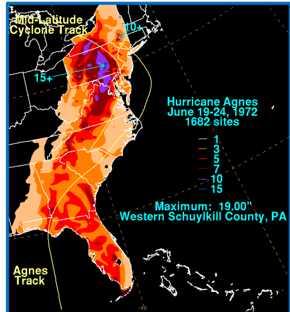
Figure 4.3.4-7 Hurricane Agnes Rainfall in Inches (NOAA WPC, n.d.)
