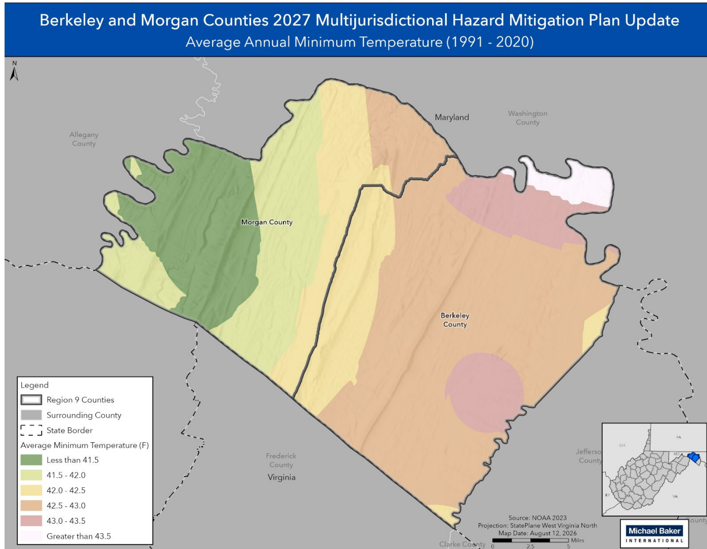
Figure 4.3.3-3: The Average Annual Minimum Temperature in Berkeley and Morgan Counties from 1991-2020.
