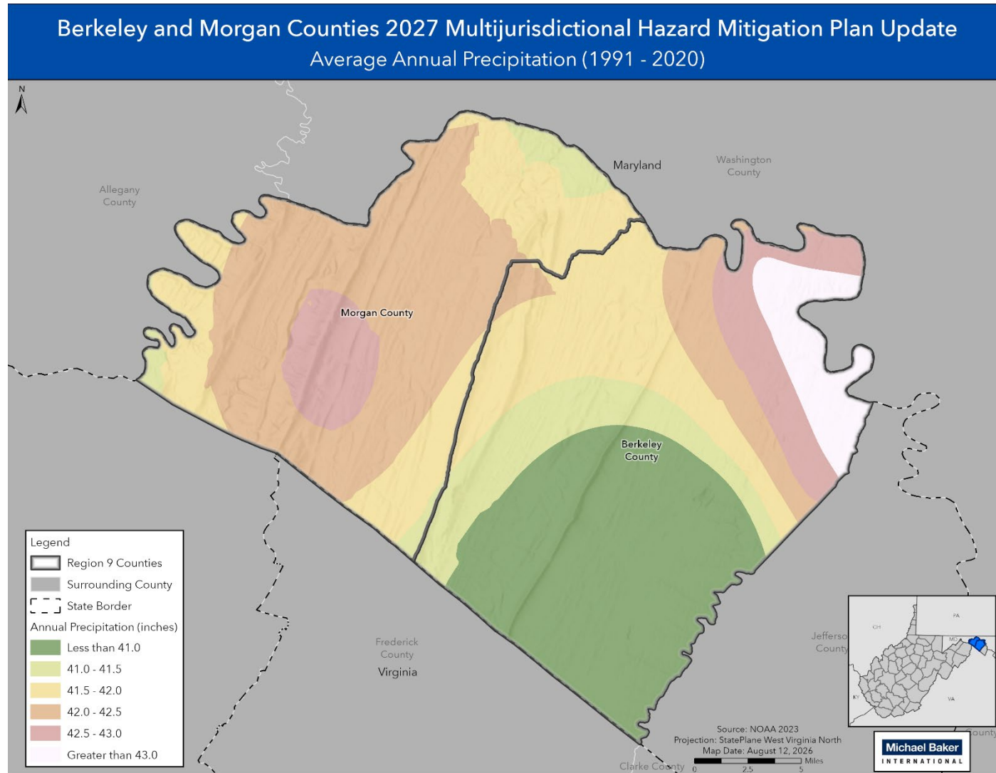
Figure 2.1-3 The Average Annual Precipitation in Berkeley and Morgan Counties from 1991 to 2020.
