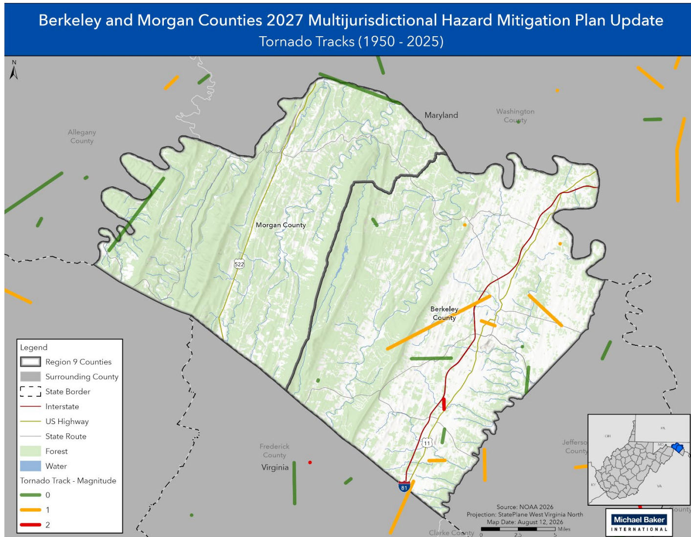
Figure 4.3.13-4 Tornado Tracks in Berkeley and Morgan Counties.
