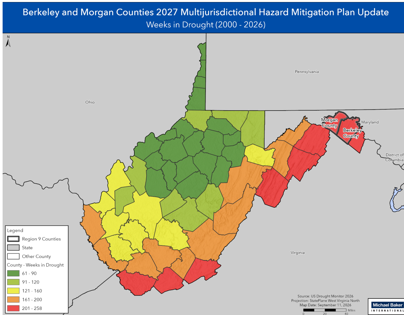
Figure 4.3.1-2 Total Weeks in Drought by County (2000 – 2026).
