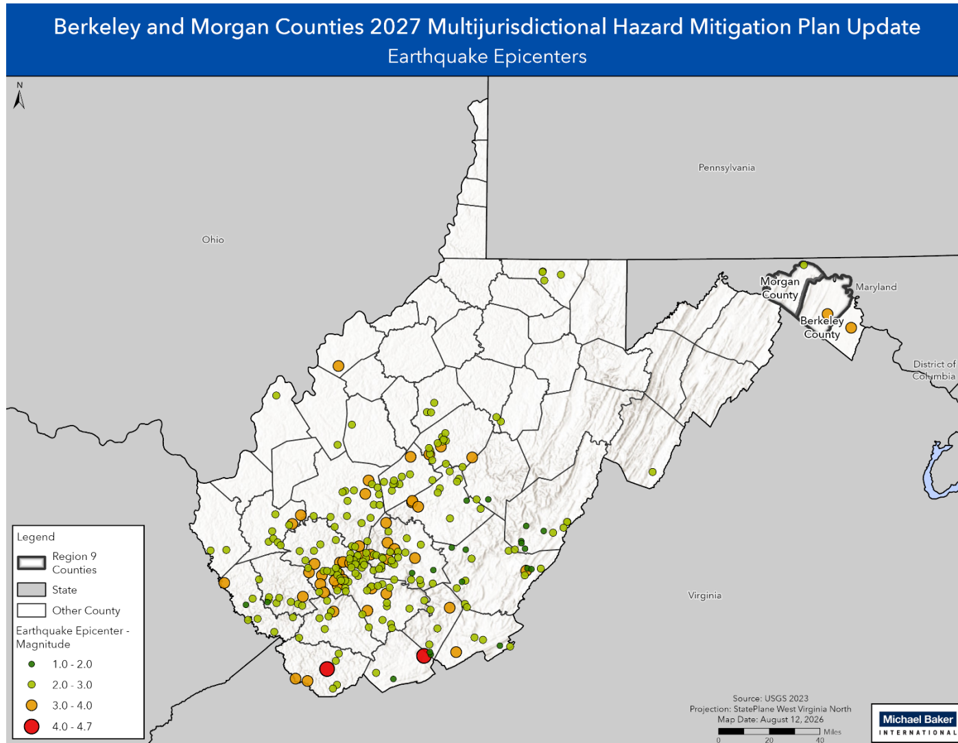
Figure 4.3.2-3 Earthquake Epicenters Throughout Berkeley and Morgan Counties and West Virginia Overall.
