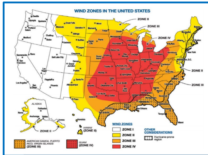
Figure 4.3.13-1 Wind Zones of the United States (IBEC, 2019)
