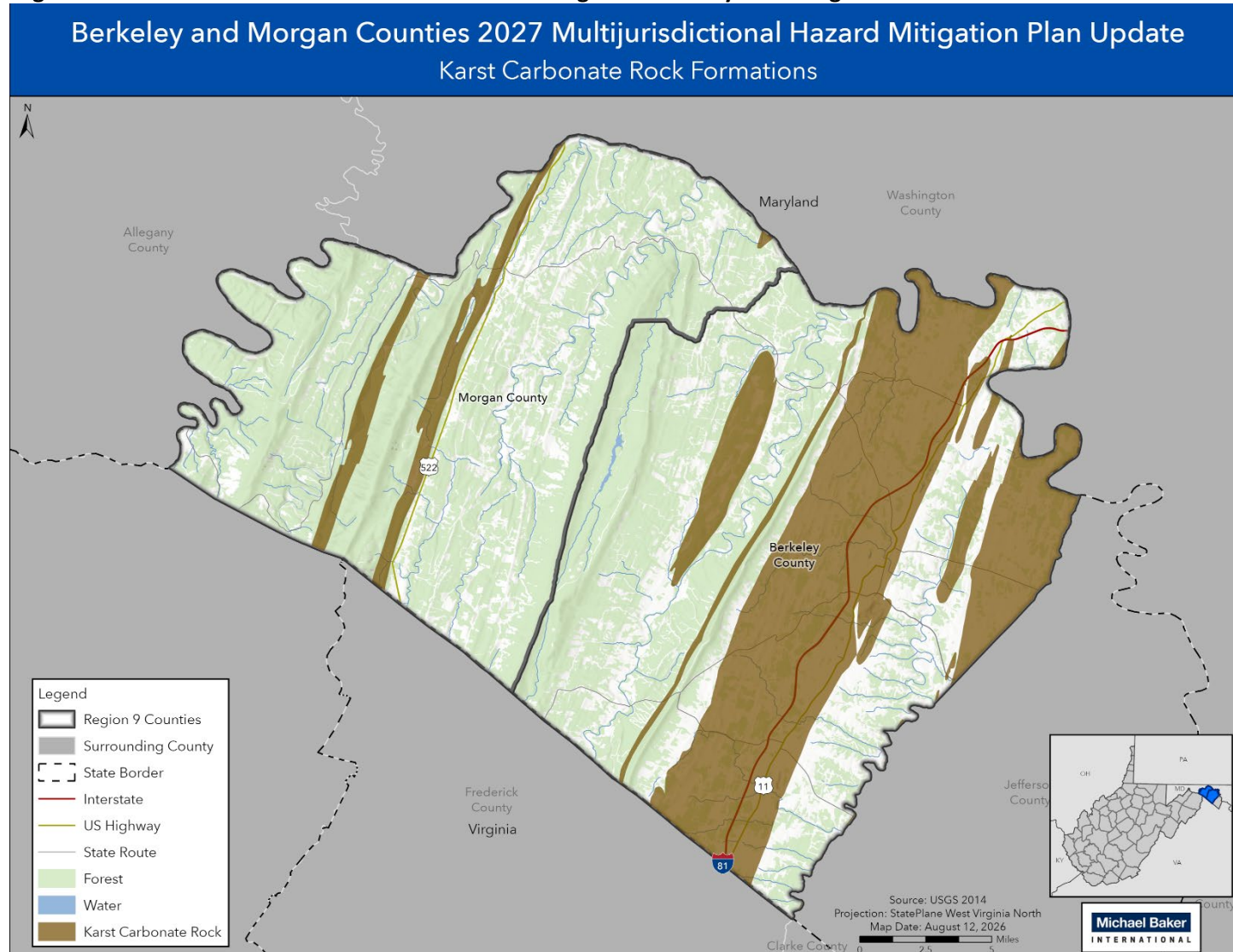
Figure 4.3.8-3 Karst Carbonate Rock Formations Throughout Berkeley and Morgan Counties.
