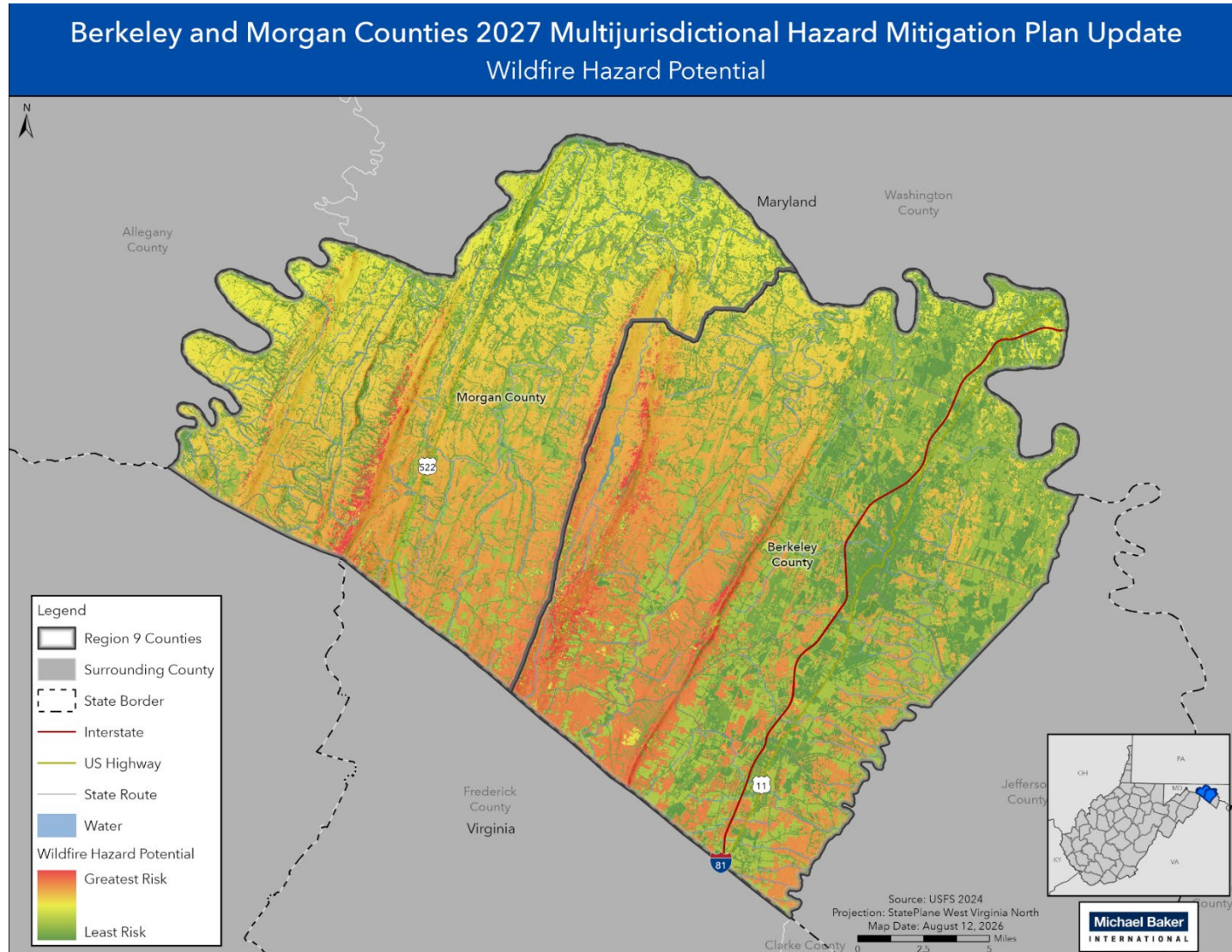
Figure 4.3.12-1 Wildfire Hazard Potential
