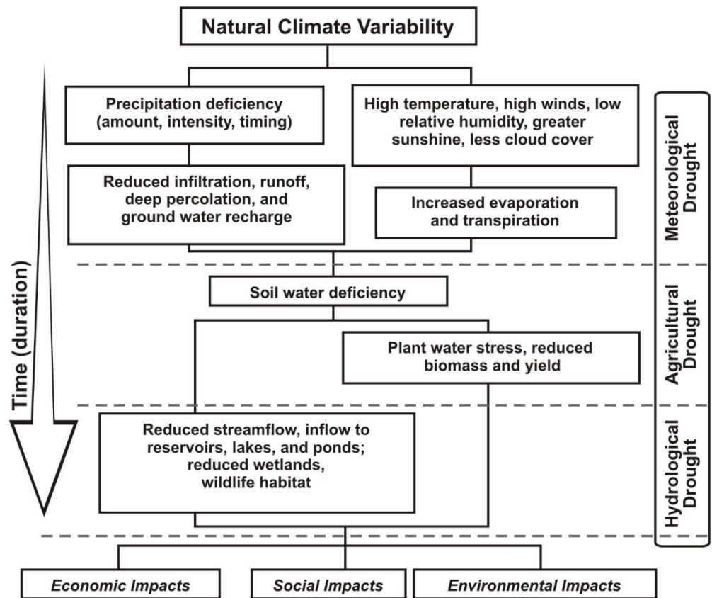
Figure 4.3.1-1: Sequence of drought occurrence and impacts for drought types (NDMC, 2026c).
