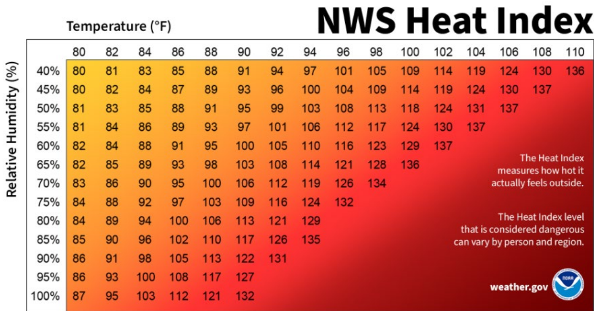
Figure 4.3.3-1 NOAA NWS Heat Index (NOAA, 2026a).
