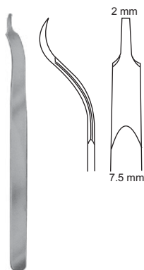
Buck-Gramcko U12-8991-15 15 cm/6"
