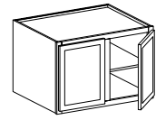
Deep Double Door 18" or 24" Height • 24" Depth 36" or *39" Width 18" Height does not have shelf
