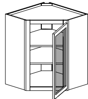
Diagonal Corner Glass Door Matching Finish Color Interior 30", 36" or 42" Height 12 or 15" Depth 24" or 27" Width
