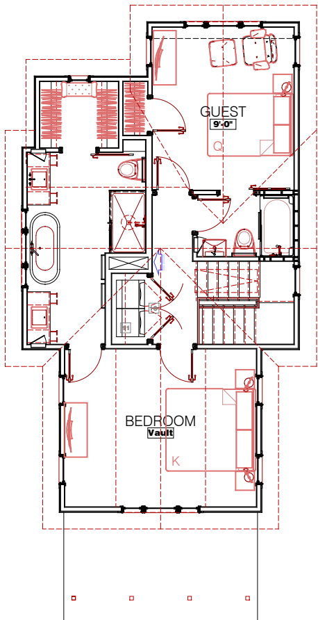
SECOND FLOOR 700sf Heated
