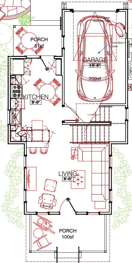
FIRST FLOOR 445sf Heated
