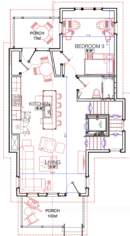
FIRST FLOOR 867sf Heated
