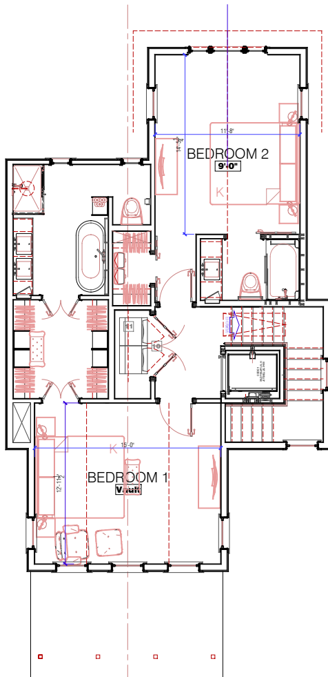
SECOND FLOOR 867sf Heated
