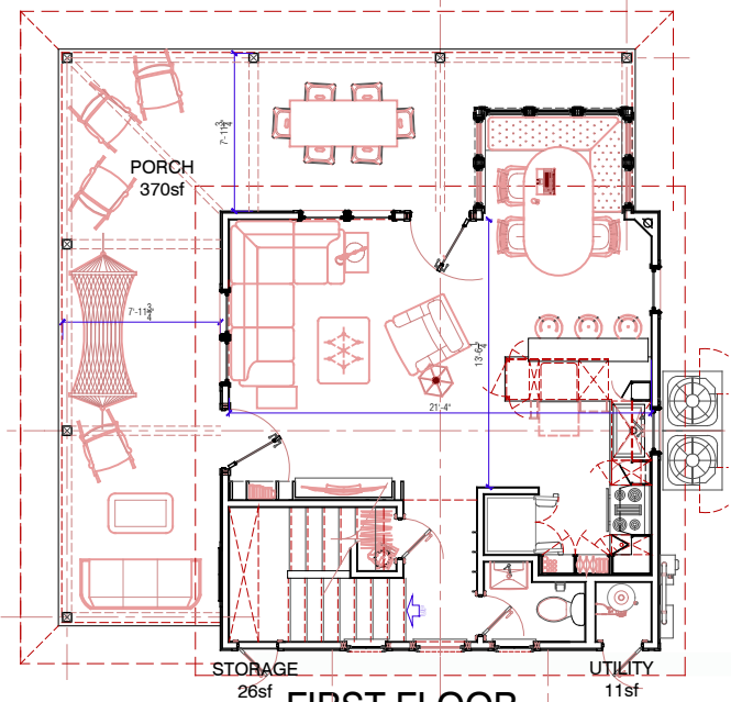
FIRST FLOOR 524sf Heated
