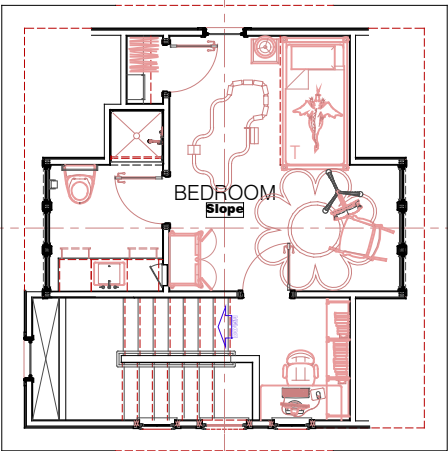
THIRD FLOOR 329sf Heated
