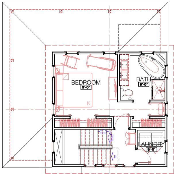
SECOND FLOOR 479sf Heated
