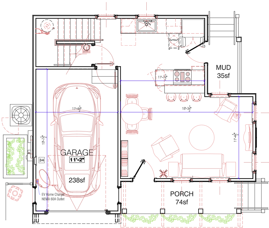
FIRST FLOOR 456sf Heated
