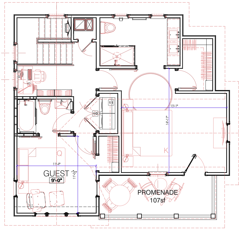
SECOND FLOOR 718sf Heated
