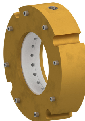
Figure 2. Solid assembled SAS drawing
