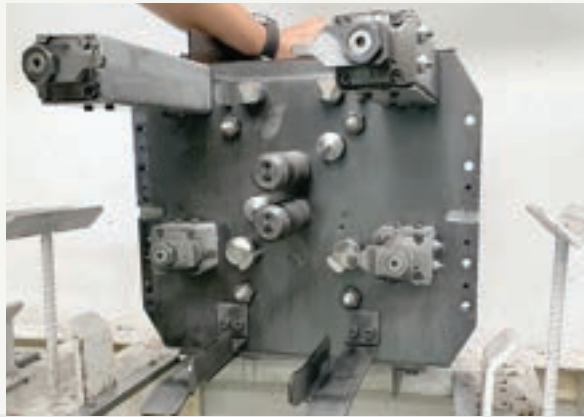
SINGLE JIG FIXTURE
