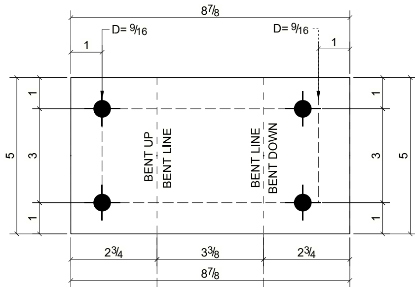
UNFOLDED VIEW
