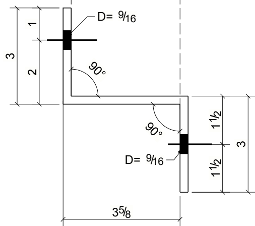
FOLDED VIEW
