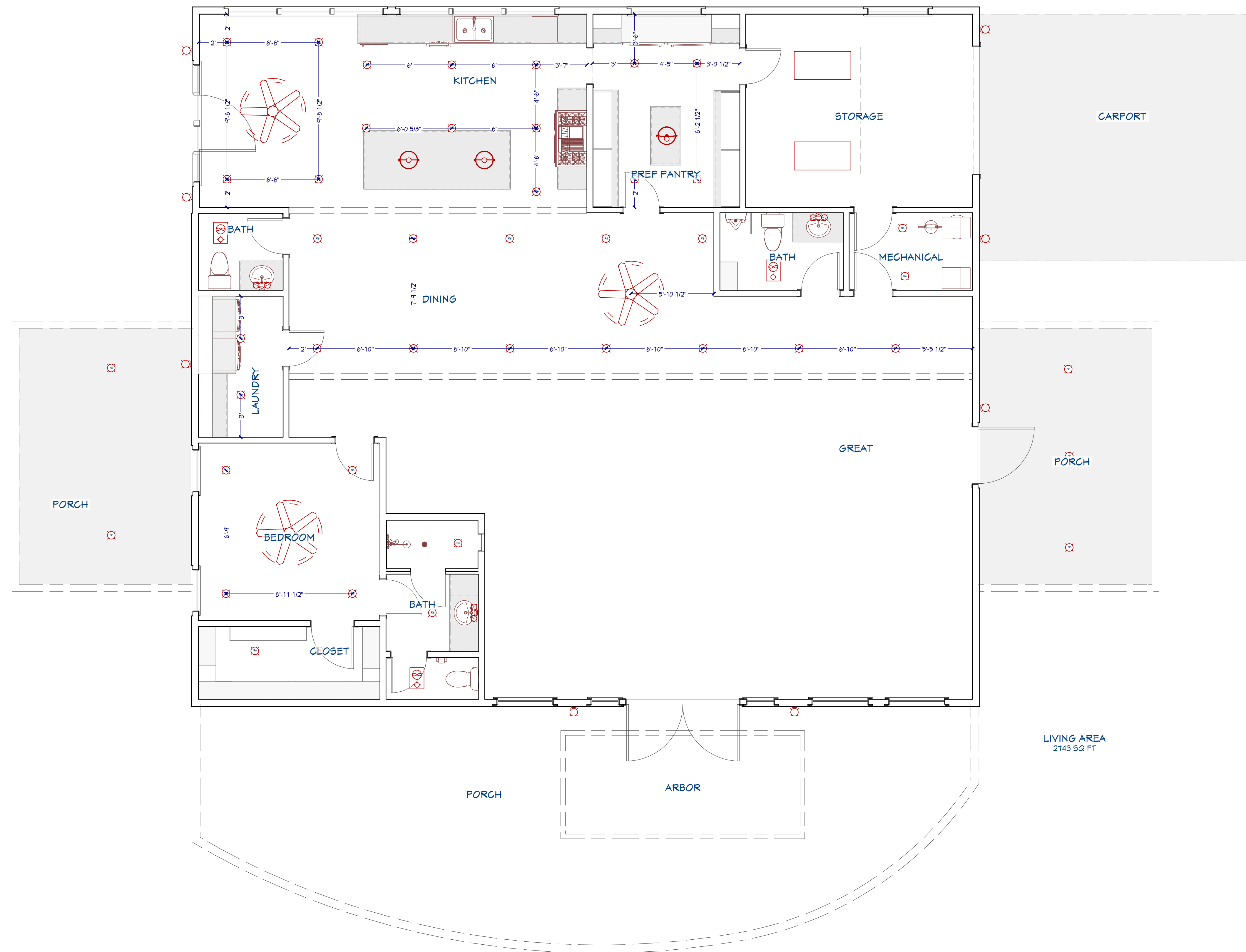
Electrical Plan View
