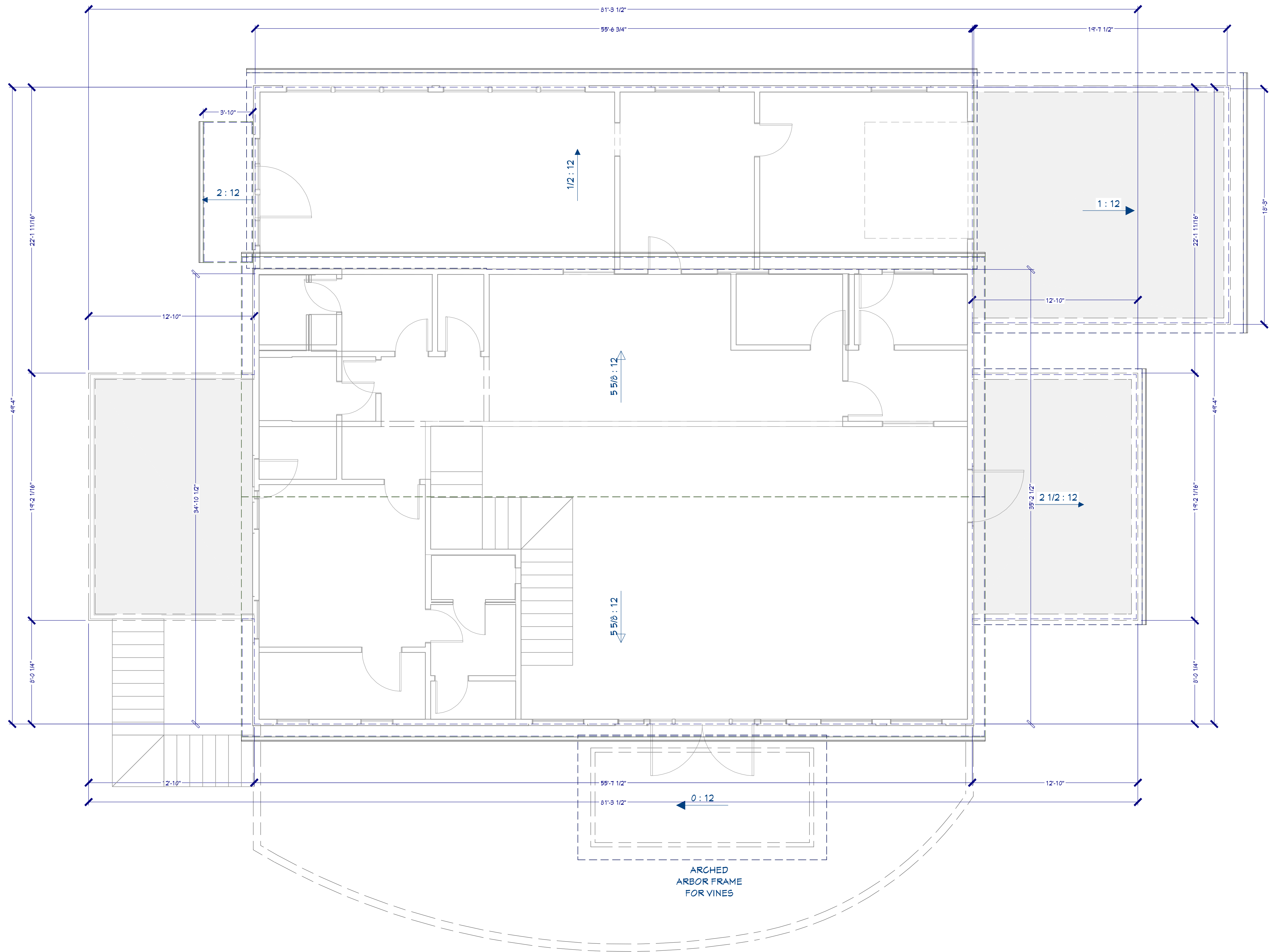
Roof Plan View
