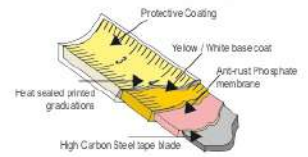
TAPE BLADE STRUCTURE
