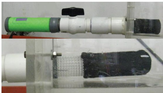
The two piece pre-filter fits snugly on a two inch outflow. The perforated tube goes onto the outflow pipe and a geotextile bag with draw strings fits over the tube.
