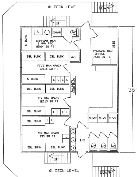
GENERAL ARRANGEMENT 01 LEVEL
