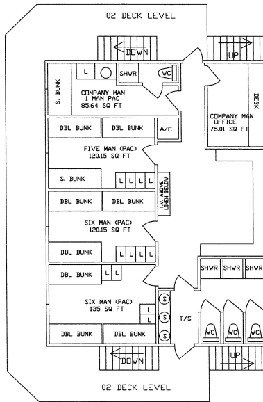
GENERAL ARRANGEMENT 02 LEVEL
