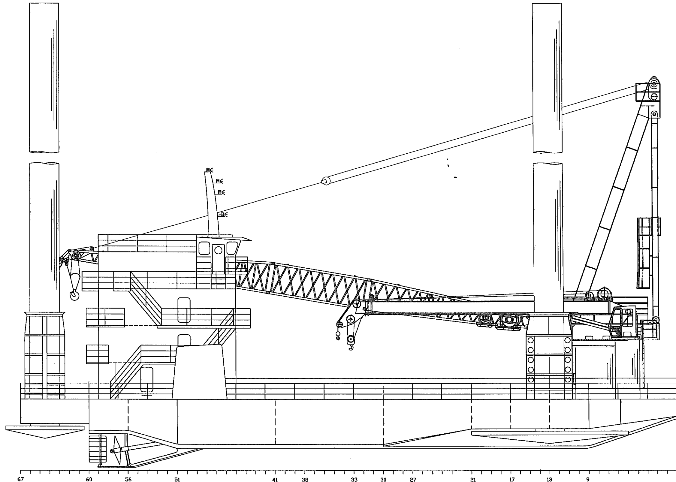
GENERAL ARRANGEMENT MAIN DECK
