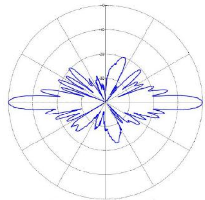
Vertical, 0° downtilt
