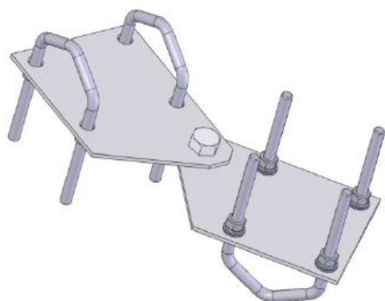
Clamp064
