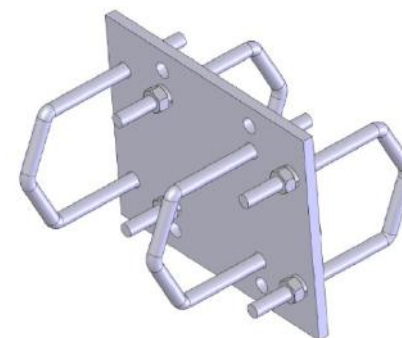
Clamp120 Parallel
