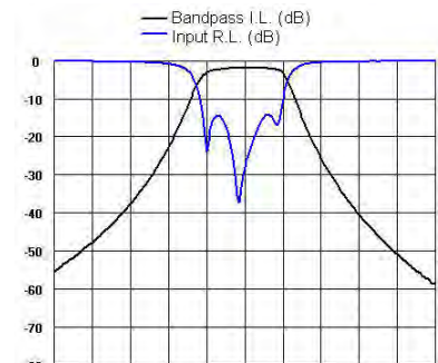
RM301-xxxSxB Preselector Response Curve
