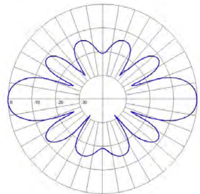
Vertical, 0° DT
