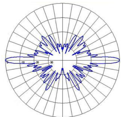
Vertical, 0° DT
