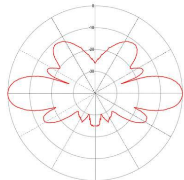
Vertical, 0° Downtilt
