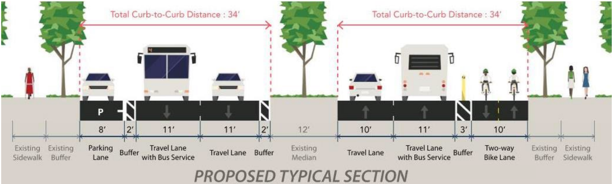
Proposed Condition
