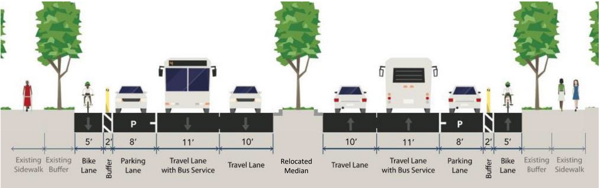
Proposed Condition
