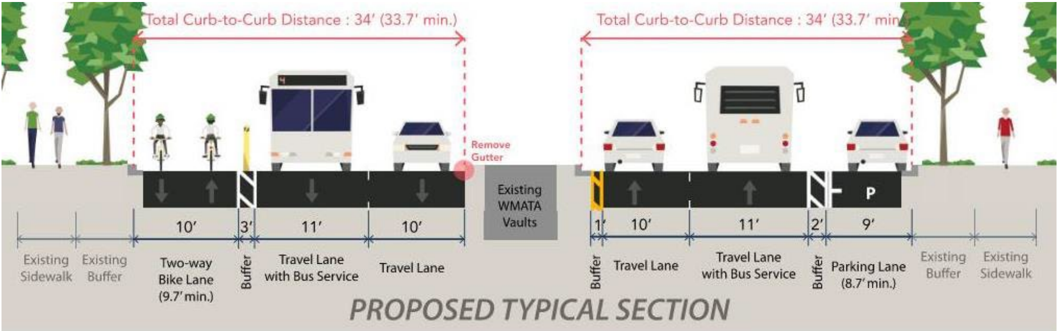
Proposed Condition
