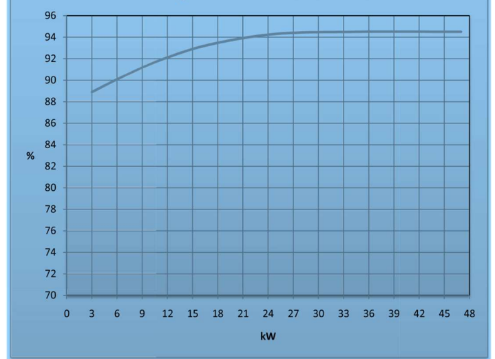
Efficiency vs Power (效率曲线)
